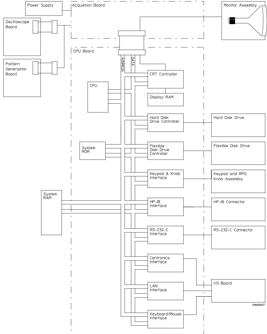
The HP 1660C/CS/CP Logic Analyzer
