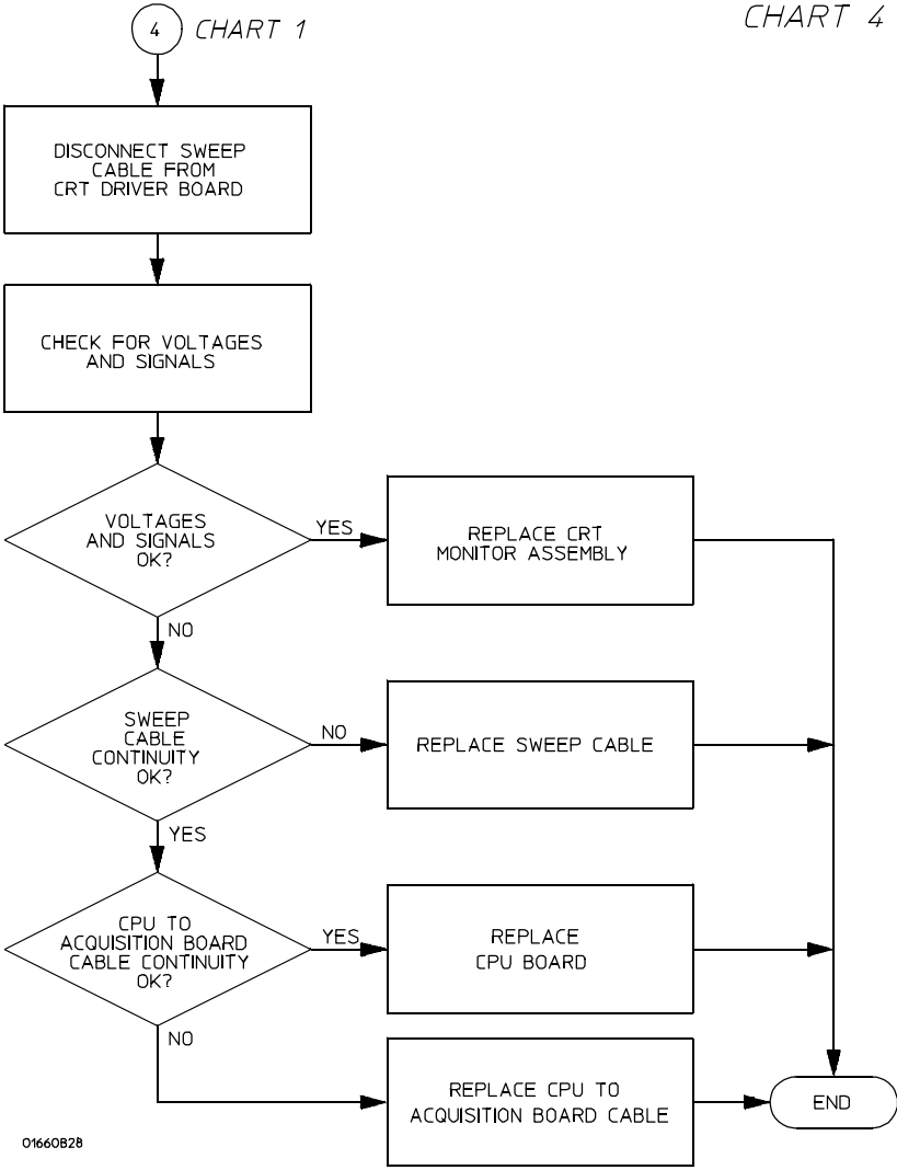
Troubleshooting Flowchart 4
