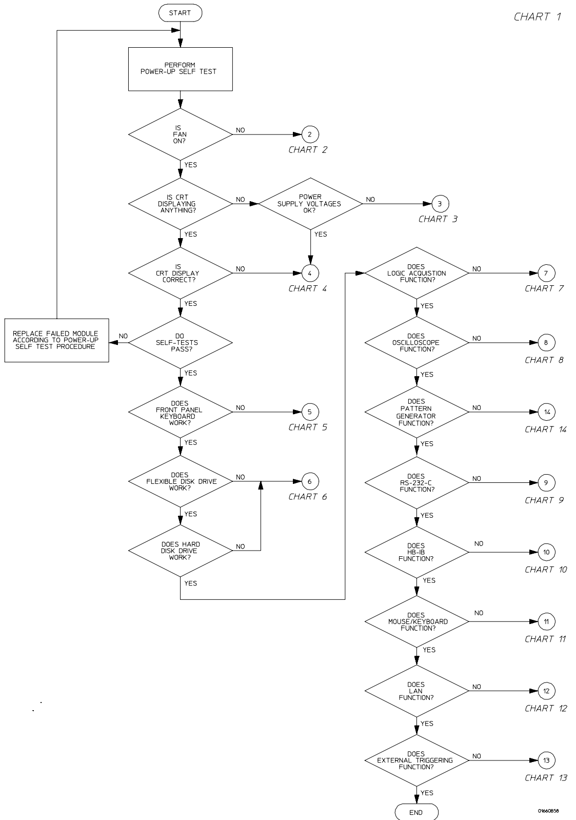
Troubleshooting Flowchart 1
