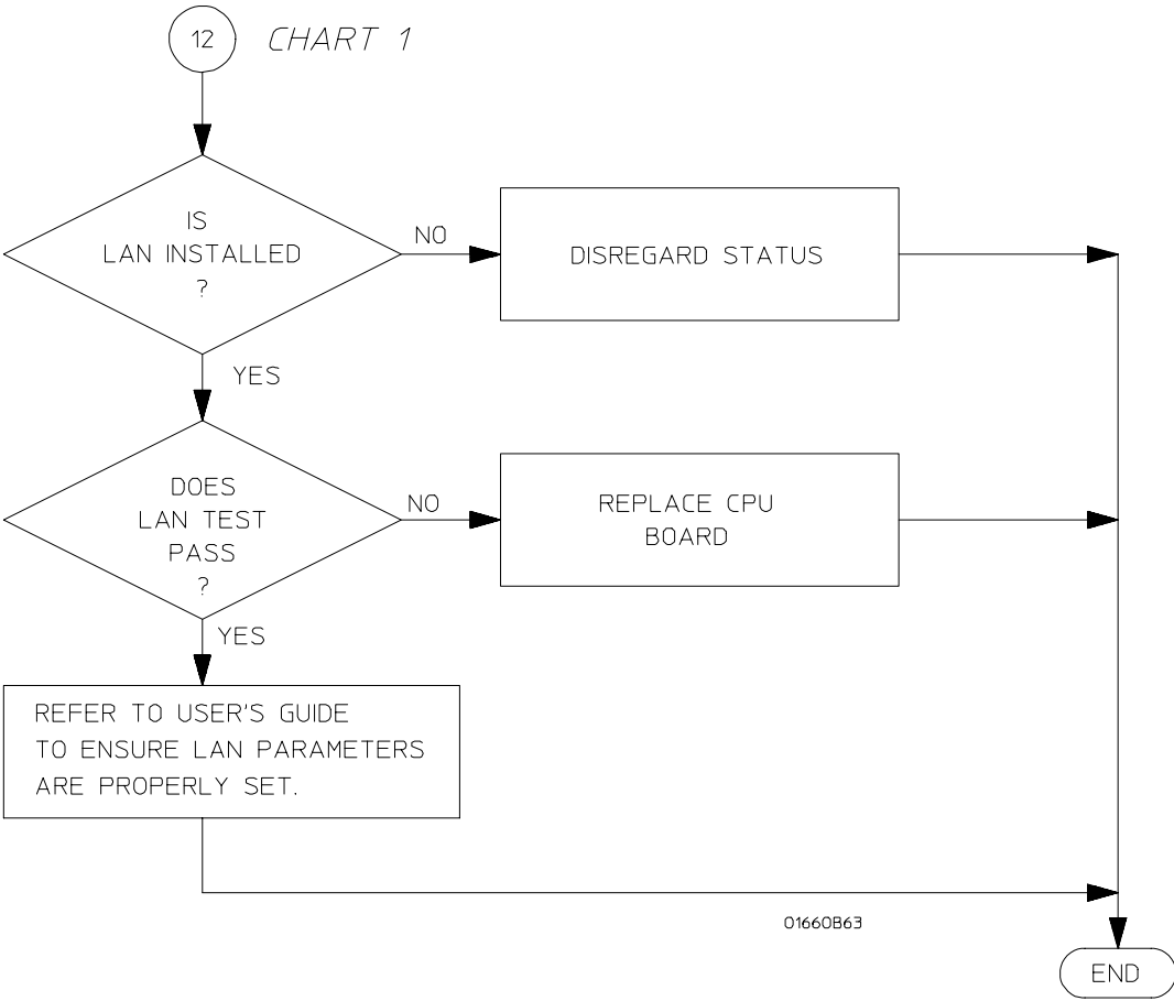
Troubleshooting Flowchart 12
