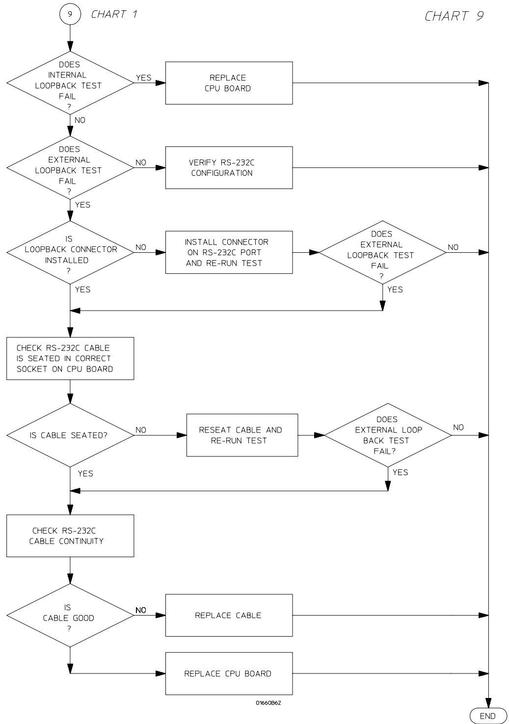
Troubleshooting Flowchart 9
